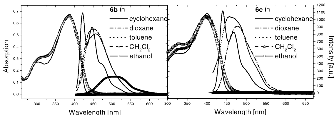
Figure 1. Solvent-dependent electronic spectra of 6b and c
